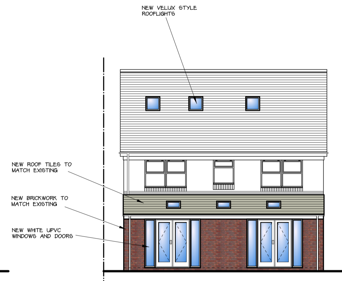
PROPOSED WEST ELEVATION (1:100)
